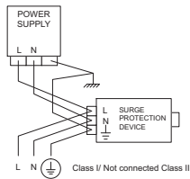
Surge Protection Device 277V
